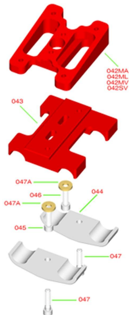
Piastra motore Engine mounting
